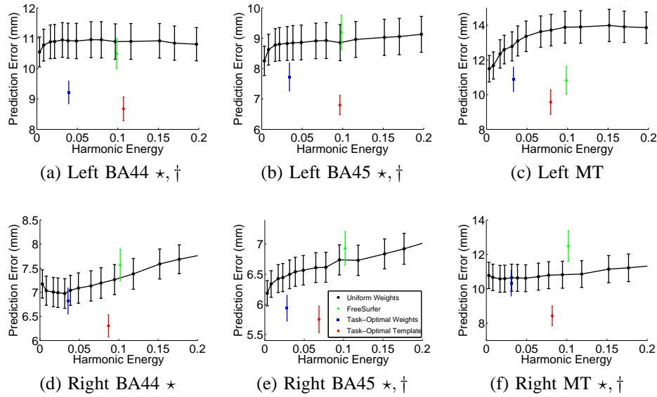
Fig. 5. Mean Hausdorff distances over an entire range of harmonic energy for BA44, BA45 and MT. First row corresponds to left hemisphere. Second row corresponds to right hemisphere. \star indicates that task-optimal template is statistically significantly better than FreeSurfer. \dagger indicates that task-optimal weights is statistically significantly better than FreeSurfer. Statistical threshold is set at 0.05, FDR corrected with respect to the 24 statistical tests performed in this section. FreeSurfer is not statistically better than either of the task-optimal methods in any of the Brodmann areas.
