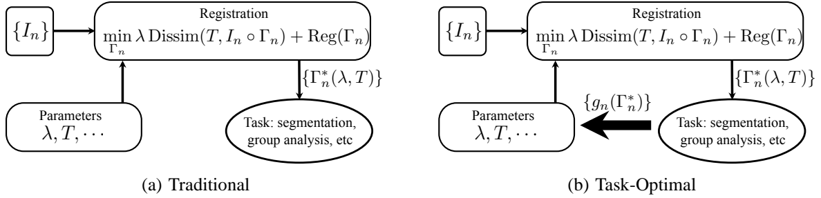
Fig. 1. Traditional and proposed frameworks for image registration. \{I_n\} indicates a collection of images. In image registration, we seek a deformation \Gamma_n^* for each image I_n . The resulting deformations \{\Gamma_n^*\} are then used for other applications, such as segmentation or group analysis. The registration cost function typically contains multiple parameters, such as the tradeoff parameter \lambda and the template T . Changes in these parameters alter the deformations \{\Gamma_n^*\} and thus the outcomes of downstream applications. In our framework (b), we assume a training data set, which allows us to evaluate the quality of the registration as measured by the application performance (or cross-validation error metric) g_n for each training subject. This allows us to pick the best parameters that result in good registration as measured by \{g_n\} . Subsequent new subjects are registered using these learned parameters.
